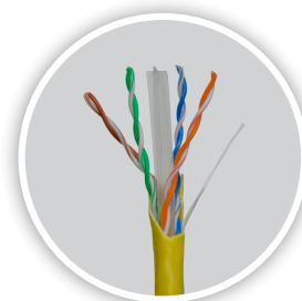
cUL/FT4 four color coded twisted pairs of 23 AWG copper wire
